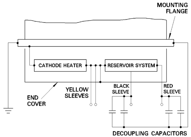
Fig. 2 CX1836X base connections
