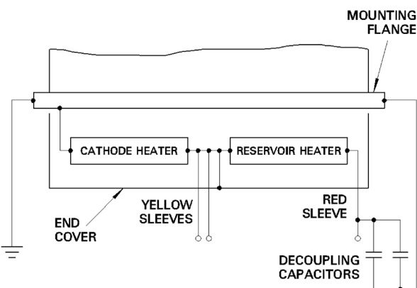
Fig. 1 CX1836 base connections
